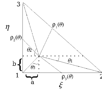
FIG. 3. A singular point in a parametric triangle.
